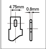
Faston T1
